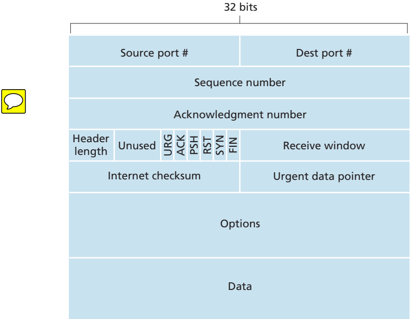
Figure 3.29 ♦ TCP segment structure
