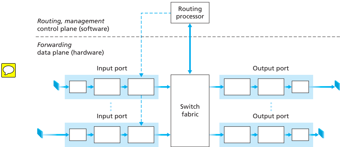
Figure 4.6 ♦ Router architecture
